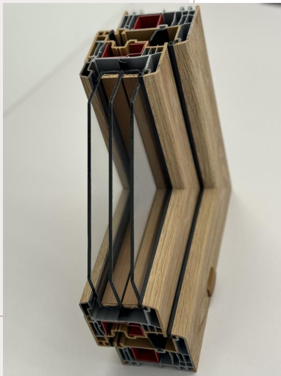
Triple glazing
